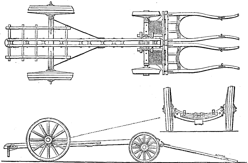
LIFE-BOAT TRANSPORTING-CARRIAGE AS ADOPTED BY THE ROYAL NATIONAL LIFE-BOAT INSTITUTION.
