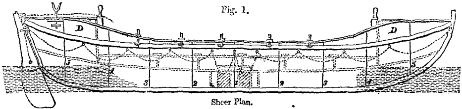
Sheer Plan.
