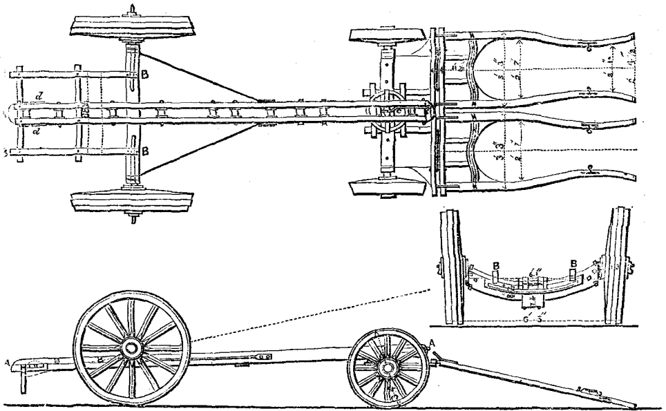
LIFE-BOAT TRANSPORTING-CARRIAGE AS ADOPTED BY THE ROYAL NATIONAL LIFE-BOAT INSTITUTION.
