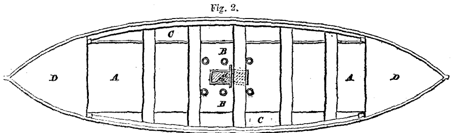
Deck Plan.
