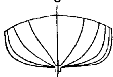
BODY PLAN
