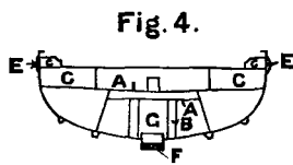
MIDSHIP SECTION.
