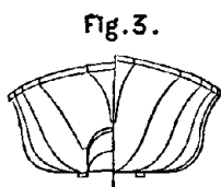
BODY PLAN
