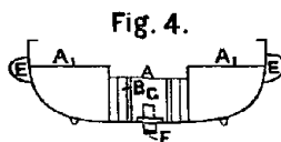
MIDSHIP SECTION
