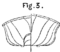
BODY PLAN
