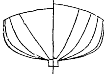
BODY PLAN
