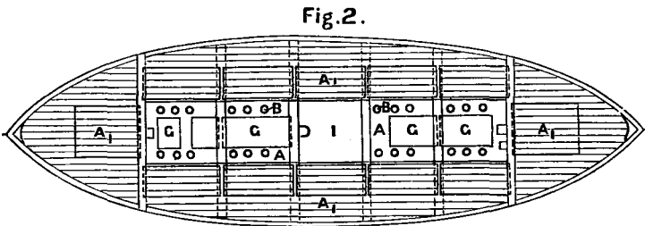
DECK PLAN
