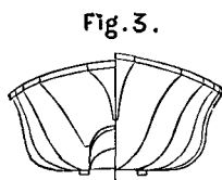
BODY PLAN
