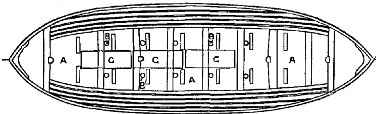
DECK PLAN.
