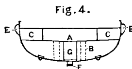
MIDSHIP SECTION.
