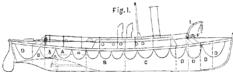
PROFILE.
