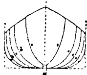
BODY PLAN
