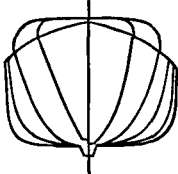
BODY PLAN
