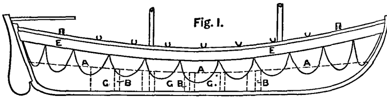
PROFILE.
