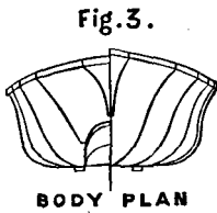
BODY PLAN
