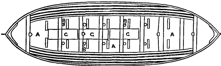
DECK PLAN.
