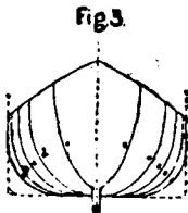
BODY PLAN
