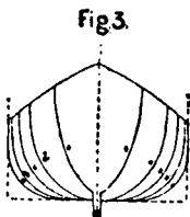
BODY PLAN
