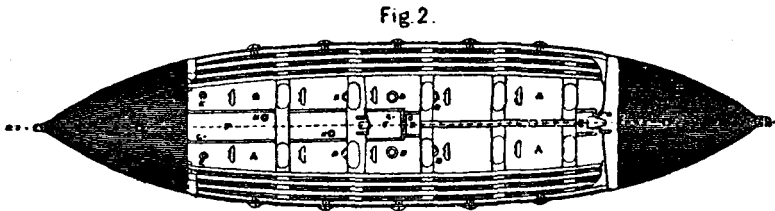
DECK PLAN.
