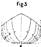
BODY PLAN
