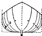
BODY PLAN
