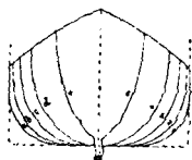
BODY PLAN
