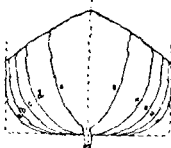
BODY PLAN
