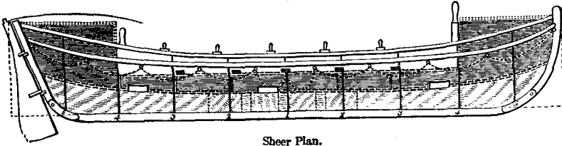
Sheer Plan.
