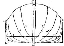
Midship Section.
