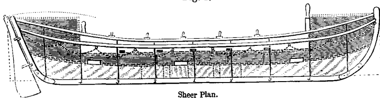
Sheer Plan.
