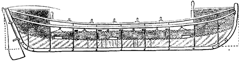
Sheer Plan.
