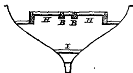
Section at 3.
