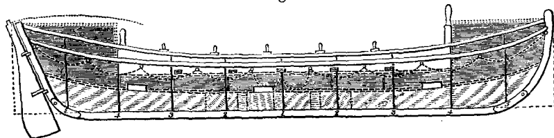
Sheer Plan.
