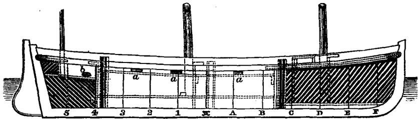
Sheer Plan.
