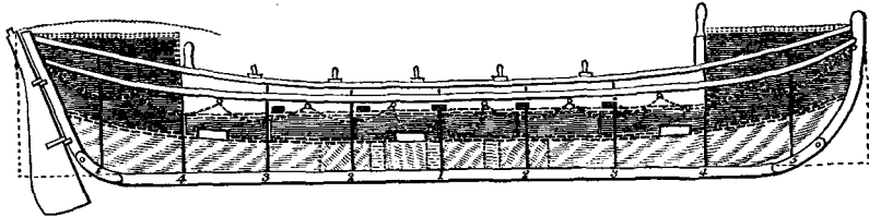
Sheer Plan.
