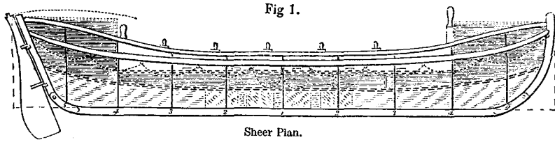
Sheer Plan.
