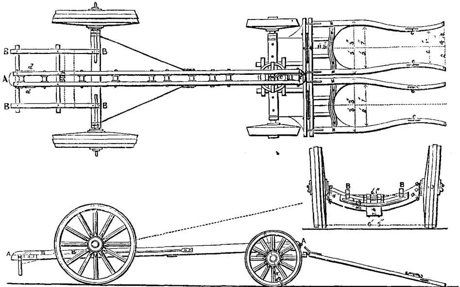
LIFE-BOAT TRANSPORTING-CARRIAGE AS ADOPTED BY THE ROYAL NATIONAL LIFE-BOAT INSTITUTION.
